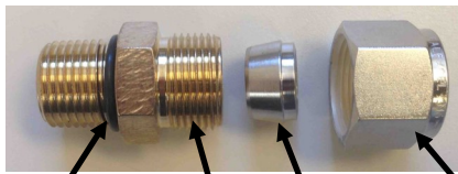
Connector O-RING Nickel-Bronze High Pressure Straight Fitting Ferrule Stainless Fitting Hex Nut
