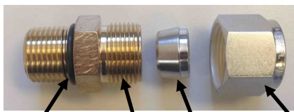
Connector O-RING
